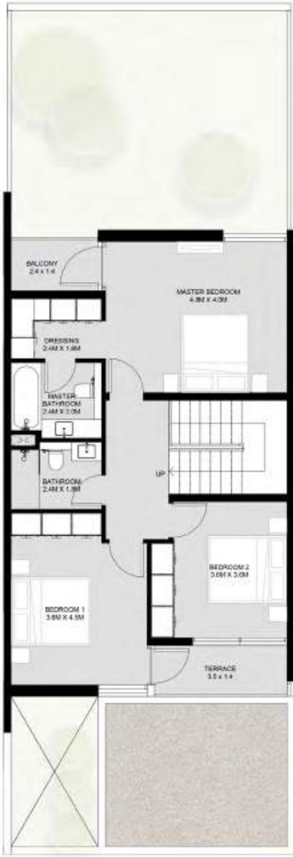
First Floor
