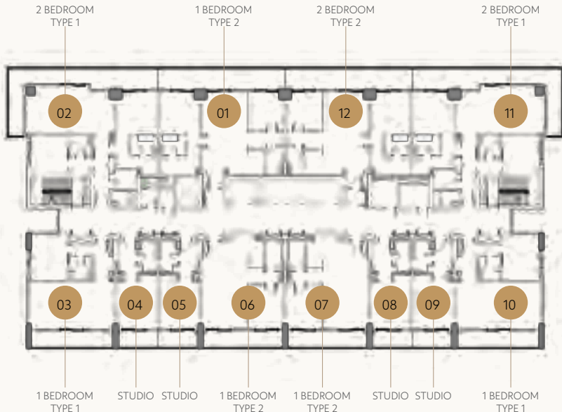
LEVELS 04-19
